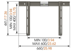
VESA mounting holes mm/inch
